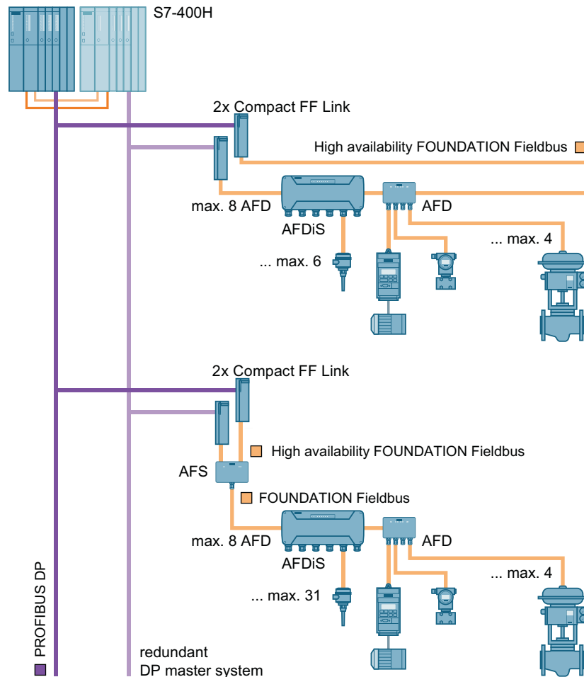
Figure 4-7 Connection to a redundant PROFIBUS DP
