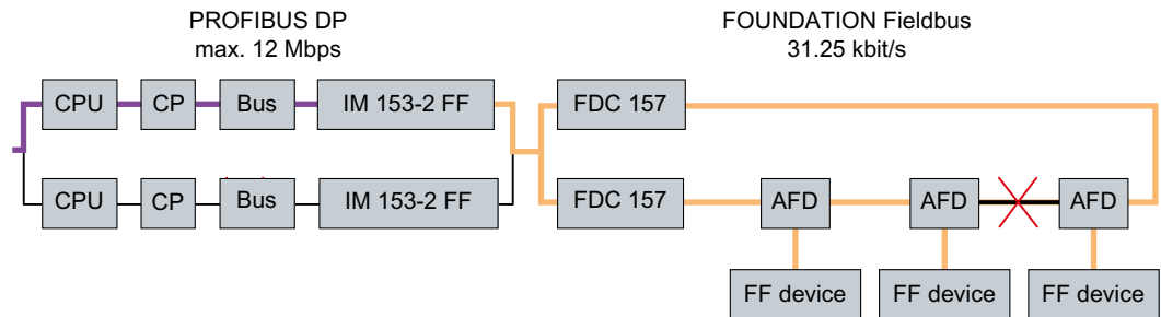
Figure 4-8 Schematic view for the installation with FF Link (2x IM 153-2 FF, 2 x FDC 157)
