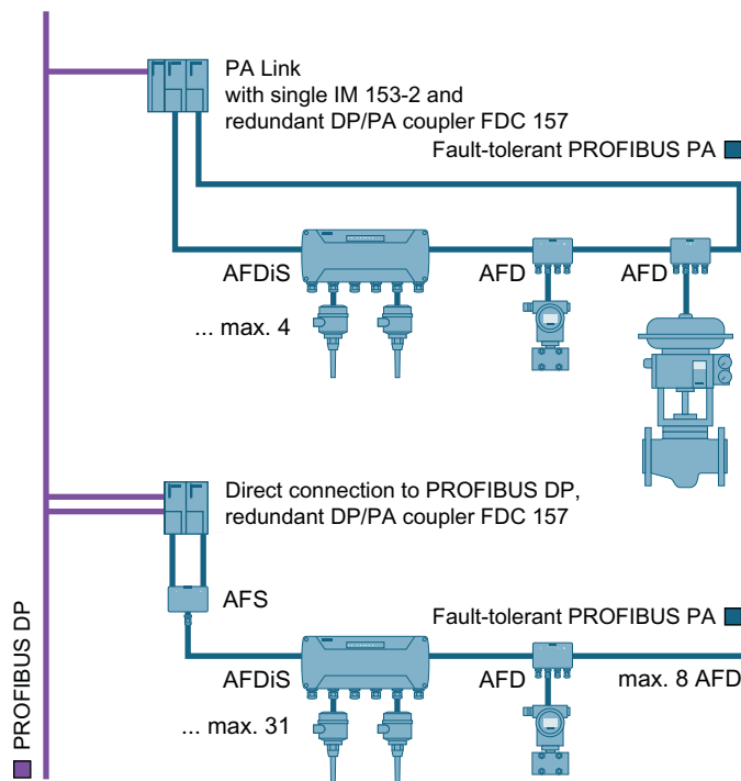
Figure 4-6 Connection to a single PROFIBUS DP
